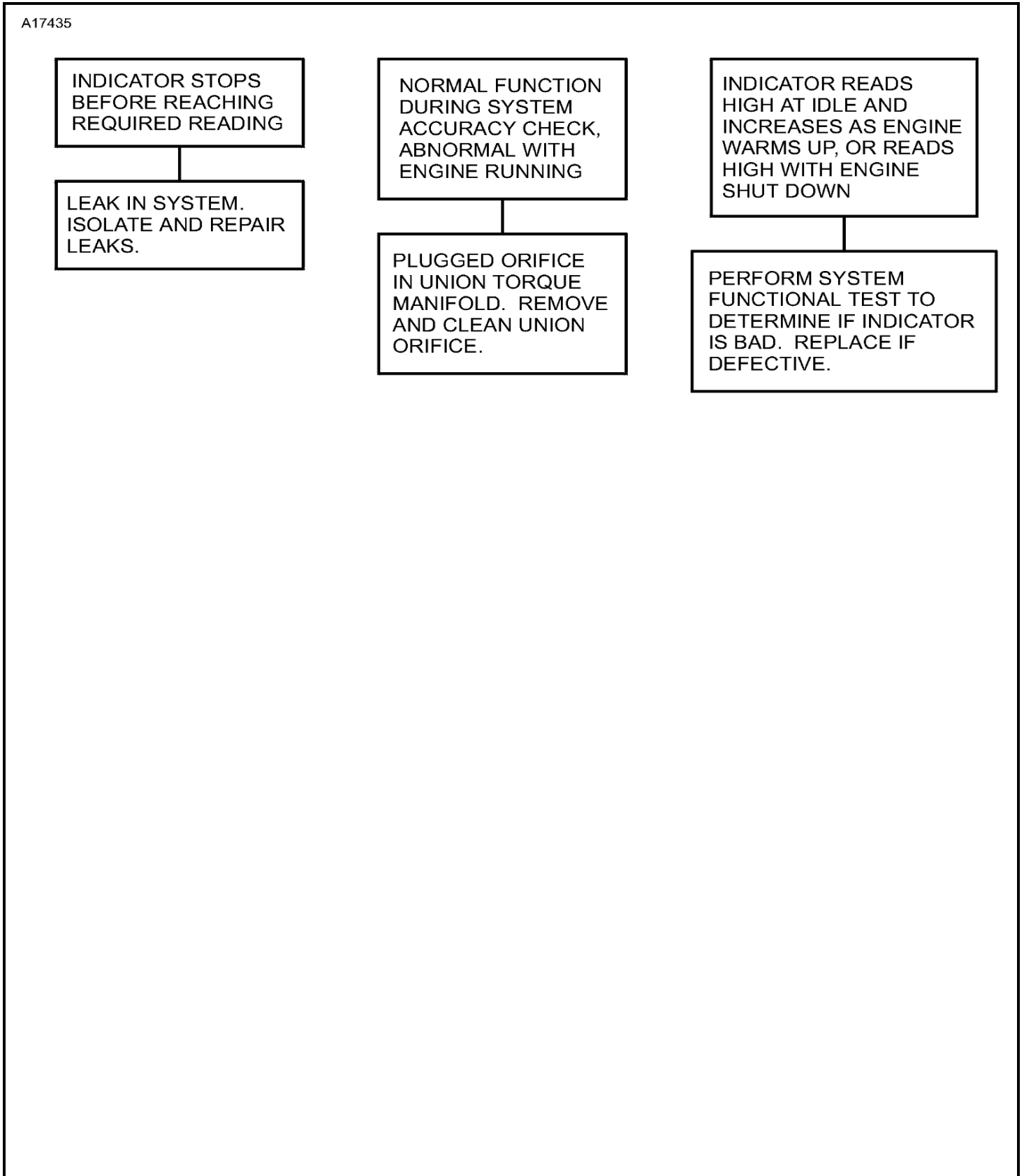
Figure 101 : Sheet 1 : Electrical Torque Indicating System Troubleshooting Chart
