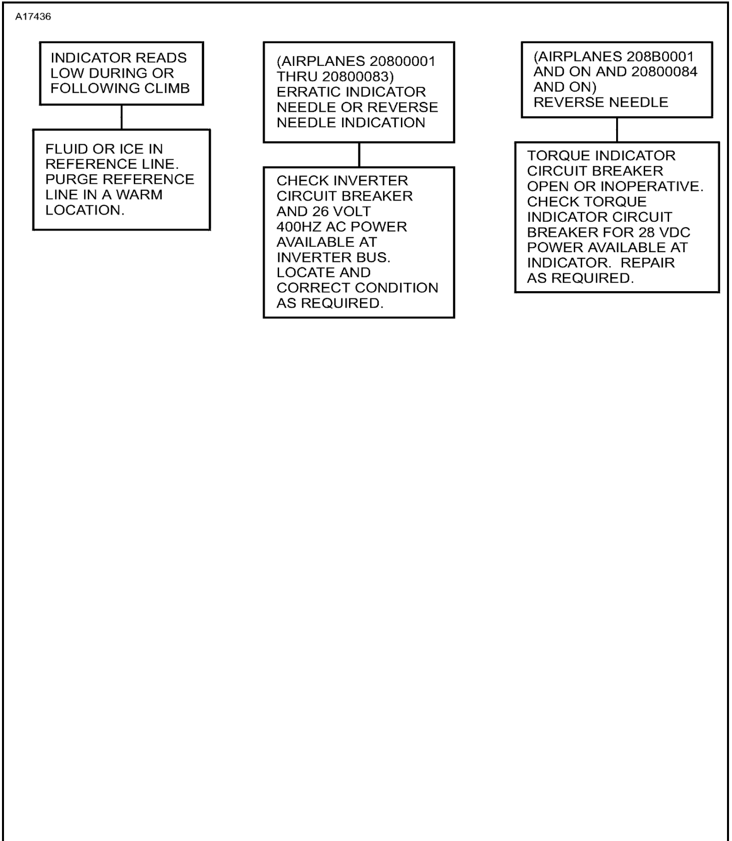
Figure 101 : Sheet 2 : Electrical Torque Indicating System Troubleshooting Chart
